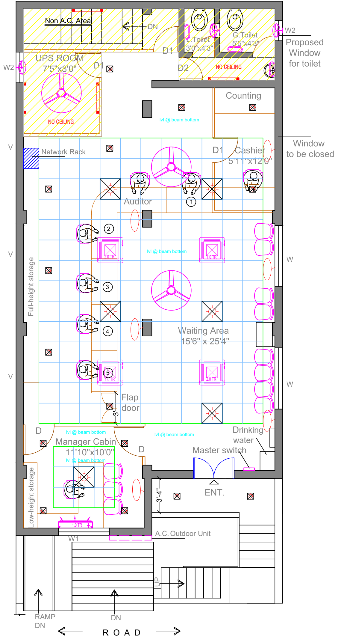
GROUND FLOOR PLAN :- Electrical Layout
