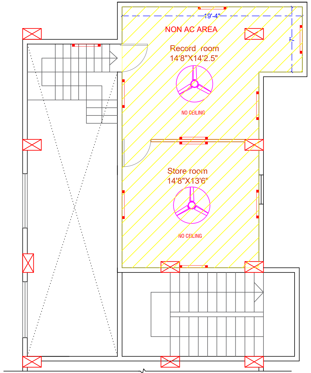
FIRST FLOOR PLAN Electrical Layout
