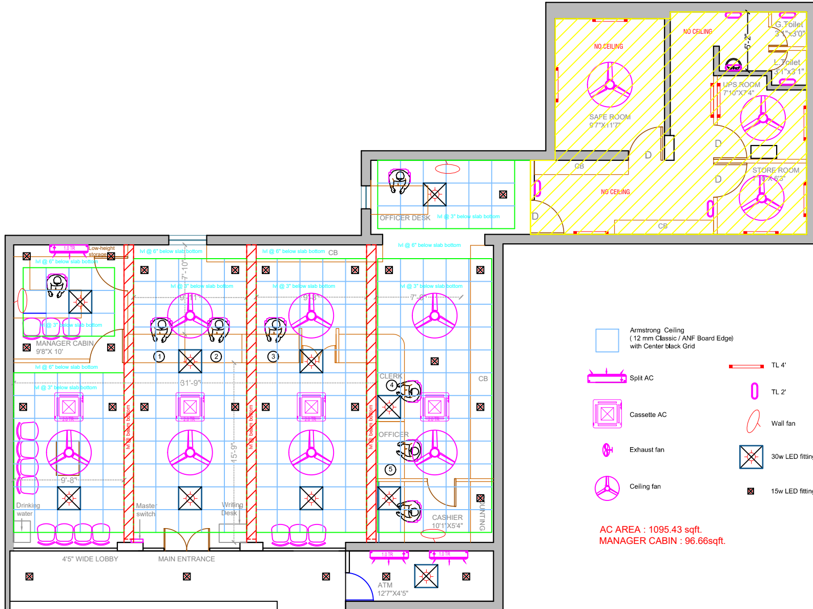
FIRST FLOOR PLAN :- Electrical Layout
