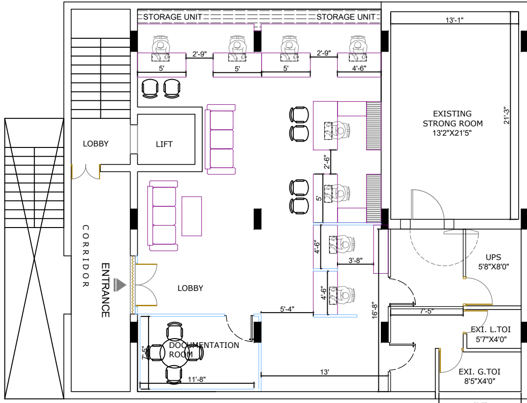
FIRST FLOOR PLAN EXISTING FLOOR
