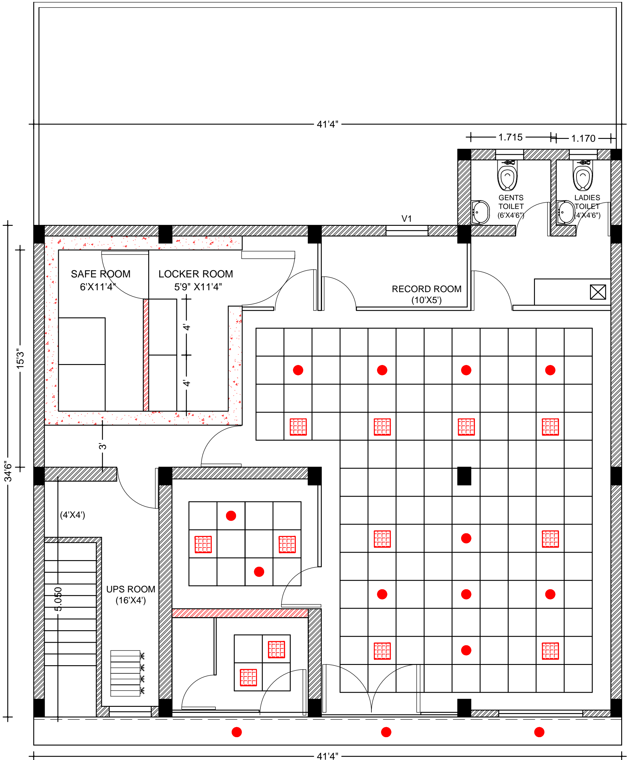
CEILING LAYOUT.LAYOUT
