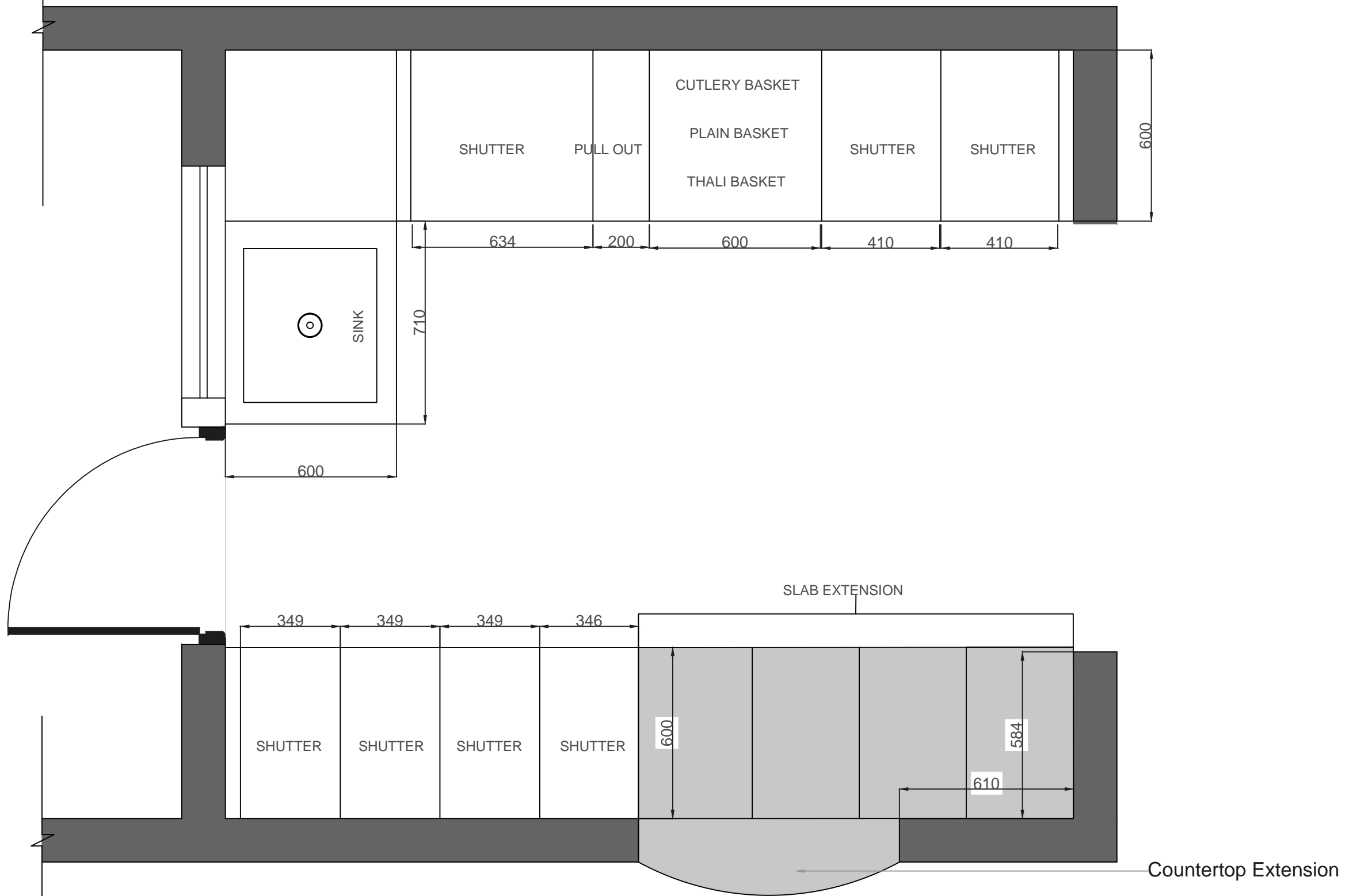
DRAWING #4 KITCHEN LAYOUT
