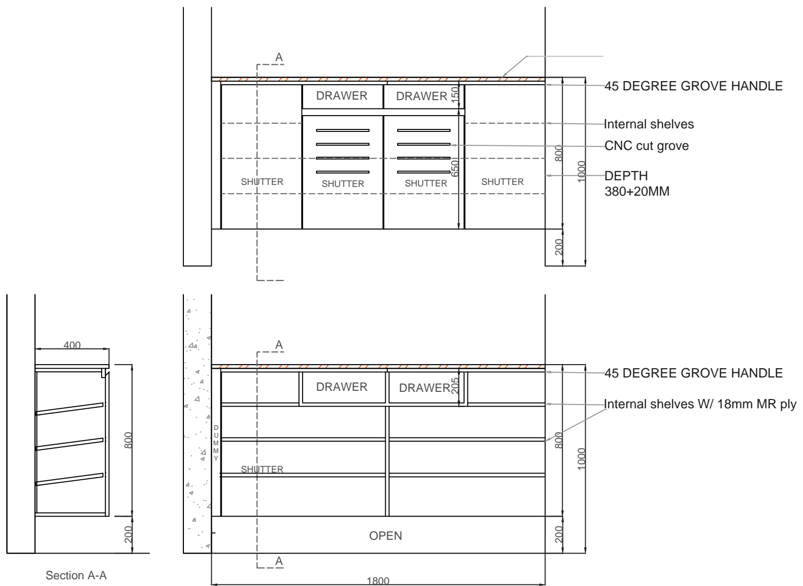
DRAWING #7 SHOE CABINET
