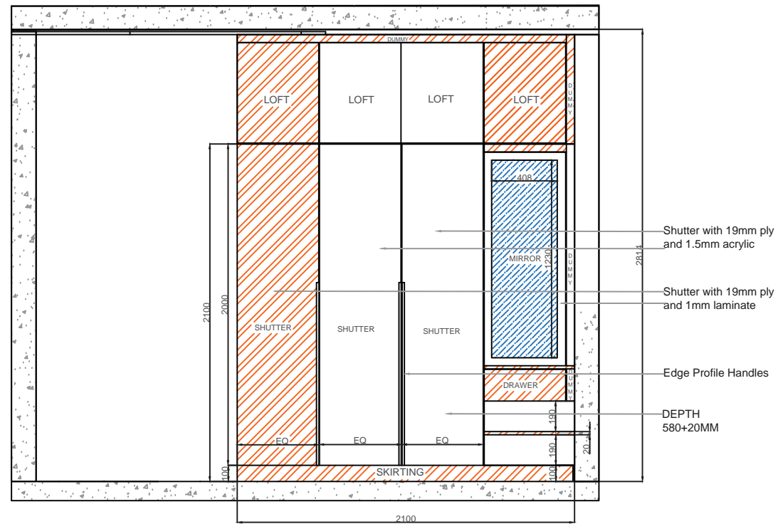
DRAWING #1 WARDROBE UNIT MASTER BEDROOM
