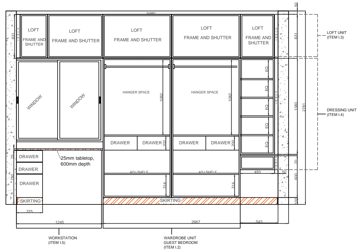
DRAWING #2 WARDROBE UNIT GUEST BEDROOM
