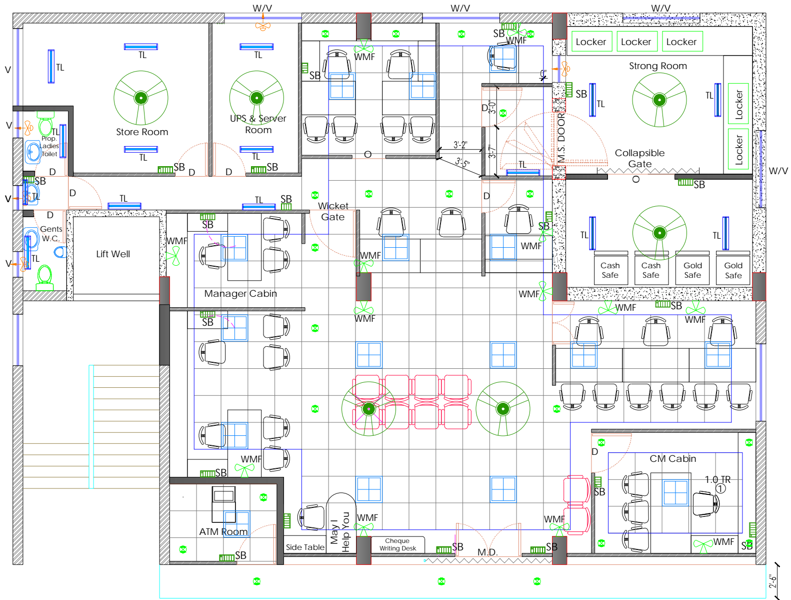
Revised Electrical Layout Plan
